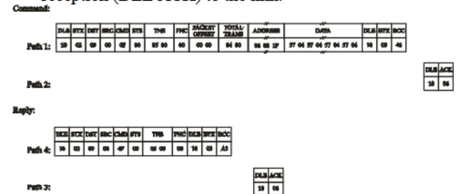
Fig. 3. Illustration of the packet exchange over the serial link
